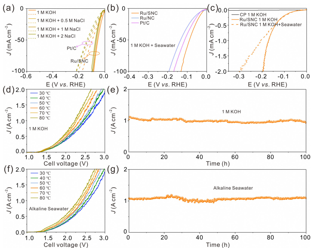
Fig. 5 (a) LSV curves of Ru/SNC spheres and Pt/C in 1 \text{ M KOH} and simulated seawater with different concentrations of NaCl. (b) LSV curves of Ru/SNC spheres, Ru/NC spheres, and Pt/C in alkaline real seawater. (c) LSV curves of CP and Ru/SNC sphere-loaded CP in 1 \text{ M KOH} and alkaline real seawater. (d) and (f) Polarization curves of the Ru/SNC||RuO 2 electrolyzer at different temperatures. (e) and (g) Stability test of the Ru/SNC||RuO 2 electrolyzer at 80 \text{ }^\circ\text{C} in 1 \text{ M KOH} (e) and alkaline real seawater (g).
