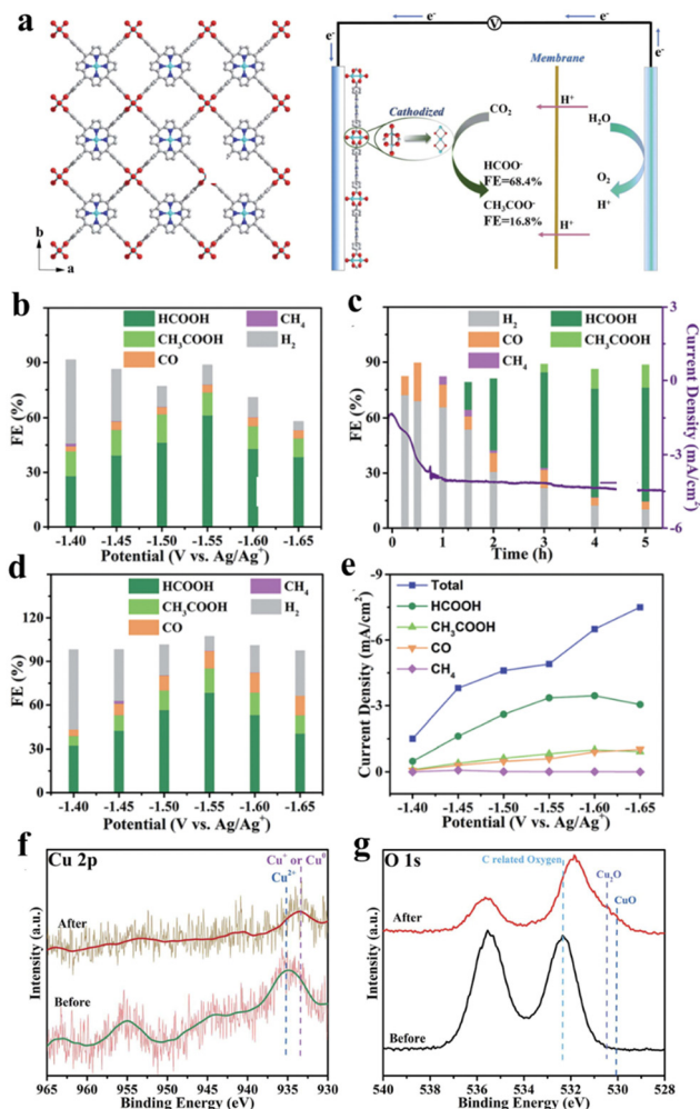
Fig. 15 (a) Crystal structure of Cu 2 (CuTCPP) nanosheets along the c axis. Red is O, blue is N, grey is Cu and cyan is C and the CO 2 electrochemical reduction system with Cu 2 (CuTCPP) nanosheets as the catalyst. (b) Faradaic efficiencies of Cu 2 (CuTCPP) nanosheets. (c) Faradaic efficiencies of Cu 2 (CuTCPP) nanosheets at different times. (d) Faradaic efficiencies of pre-electrolyzed Cu 2 (CuTCPP) nanosheets. (e) Total and partial current densities for CO 2 RR products on pre-electrolyzed Cu 2 (CuTCPP). (f) Cu 2p XPS spectra and (g) O 1s XPS spectra of Cu 2 (CuTCPP) on FTO before and after 5 h reaction. All potentials were set at -1.55 V vs. Ag/Ag + . Reproduced from ref. 145. Copyright 2022 RSC.
