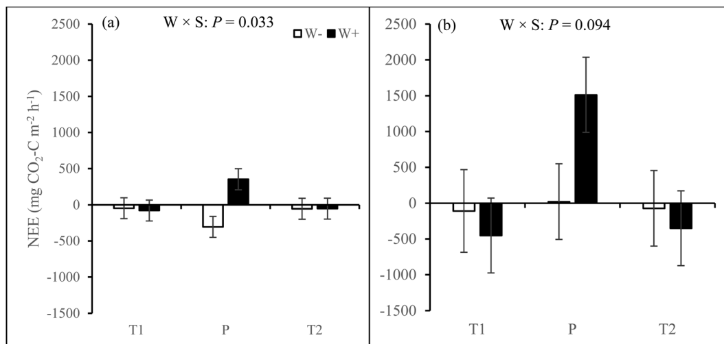
Fig. 2 Net ecosystem exchange (NEE) in mesocosms from T1, T2, and P sites under treatments with warming ( W+ , i.e. warming only and warming + increased cloudiness treatments) and without warming ( W- , i.e. control and increased cloudiness only treatments) across five measurement campaigns in (a) the first and (b) second growing seasons. Bars represent season mean values ( \pm SE, n = 10 per site per treatment). T = tundra, where T1 and T2 indicate the two locations within the tundra, and P = palsa mire. W \times S = warming \times site interaction. Statistically significant P -values < 0.05 and marginally significant P -values < 0.1 from LMM ANOVA are shown. See ESI_1 Tables S3 and S4† for detailed statistics.
