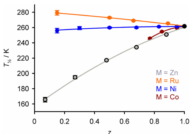
Fig. 3 Variation of T_{1/2} with composition in [\text{Fe}_2\text{M}_{1-z}(\text{1-bpp})_2][\text{BF}_4]_2 (Scheme 1) with different dopant ions. The \text{Fe}_2\text{Zn}_{1-z} data correspond to those in Fig. 2. Analogous data for other doped SCO compounds are in Fig. S1 and S2.† This figure has been adapted from ref. 63 with permission from the Royal Society of Chemistry, copyright 2023.
