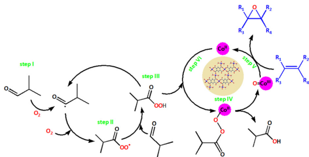
Fig. 9 Possible reaction mechanism steps for the formation of peroxy species catalysed by the heterogeneous catalyst 2 in the epoxidation of olefins. \{Co(OH_2)_2O_4\} active species is represented by Co II .
