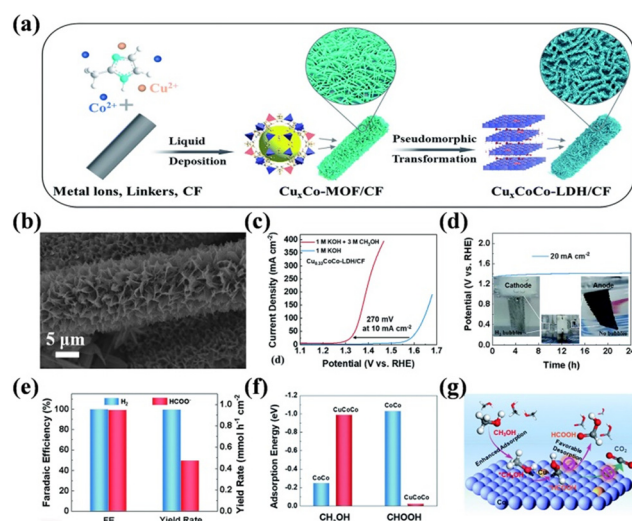
Fig. 9 (a) Schematic illustration of the fabrication of \text{Cu}_x\text{CoCo-LDHs/CF} . (b) SEM image of \text{Cu}_{0.33}\text{CoCo-LDHs/CF} . (c) Polarization curves of \text{Cu}_{0.33}\text{CoCo-LDH/CF} in 1 \text{ M KOH} or 1 \text{ M KOH} + 3 \text{ M CH}_3\text{OH} solution. (d) Chronopotentiometry curve of \text{Cu}_{0.33}\text{CoCo-LDH/CF} in 1 \text{ M KOH} + 3 \text{ M CH}_3\text{OH} solution at 20 \text{ mA cm}^{-2} . (e) Comparison of the FE and yield rate for formate and \text{H}_2 on \text{Cu}_{0.33}\text{CoCo-LDH/CF} . (f) Calculated adsorption energy of methanol and formate molecules on the surfaces of \text{CoCo-LDH} and \text{CuCoCo-LDH} . (g) Schematic process for the transformation of \text{CH}_3\text{OH} molecules into \text{HCOOH} instead of \text{CO}_2 on the surface of \text{CuCoCo-LDH} . 154 Reproduced from ref. 154 with permission from the Royal Society of Chemistry, Copyright 2022.
