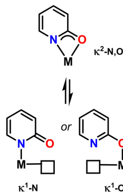
Scheme 1 Coordination bonding motifs of the 2-pyridone/2-pyridonate ligand platform.
