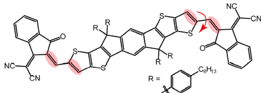
(a) Photochemical stability of ITIC under N 2 atmosphere
