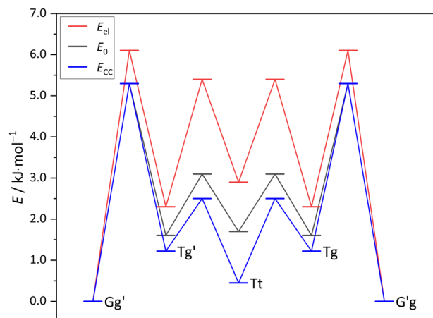
Fig. 6 Cl monomer energies for minima and transition states (Tables S6, S7 and Fig. S2 in the ESI † ) at B3LYP-D3(BJ)/def2-QZVP level without ZPVE ( E_{el} ), with ZPVE ( E_0 ) and with the electronic energy being replaced by the DLPNO-CCSD(T)/aug-cc-pVQZ//B3LYP-D3(BJ)/def2-QZVP value ( E_{cc} ).
