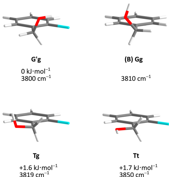
Fig. 5 Optimised Cl monomer structures (Tables S3–S5, ESI † ) with harmonically zero-point-corrected relative energies and unscaled harmonic OH stretching wavenumbers at B3LYP-D3(BJ)/def2-QZVP level. The Br and I monomers show analogous structures but different relative energies (Fig. 7). The Gg conformation of B monomer is shown for comparison.
