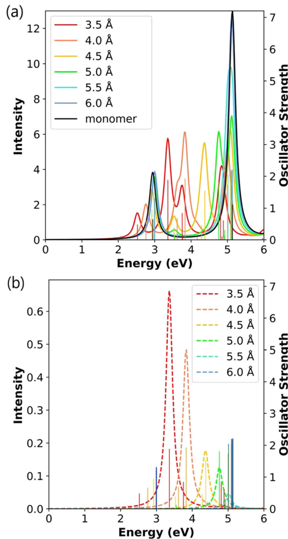
Fig. 7 (a) Absorption spectra and (b) CTP absorption spectra of the side-by-side \text{Ag}_2 nanowire dimers at the INDO/CIS level. The absorption intensity of the monomer is doubled to represent the intensity for two isolated monomers. In both panels, the sticks indicate the oscillator strength of each excited state.
