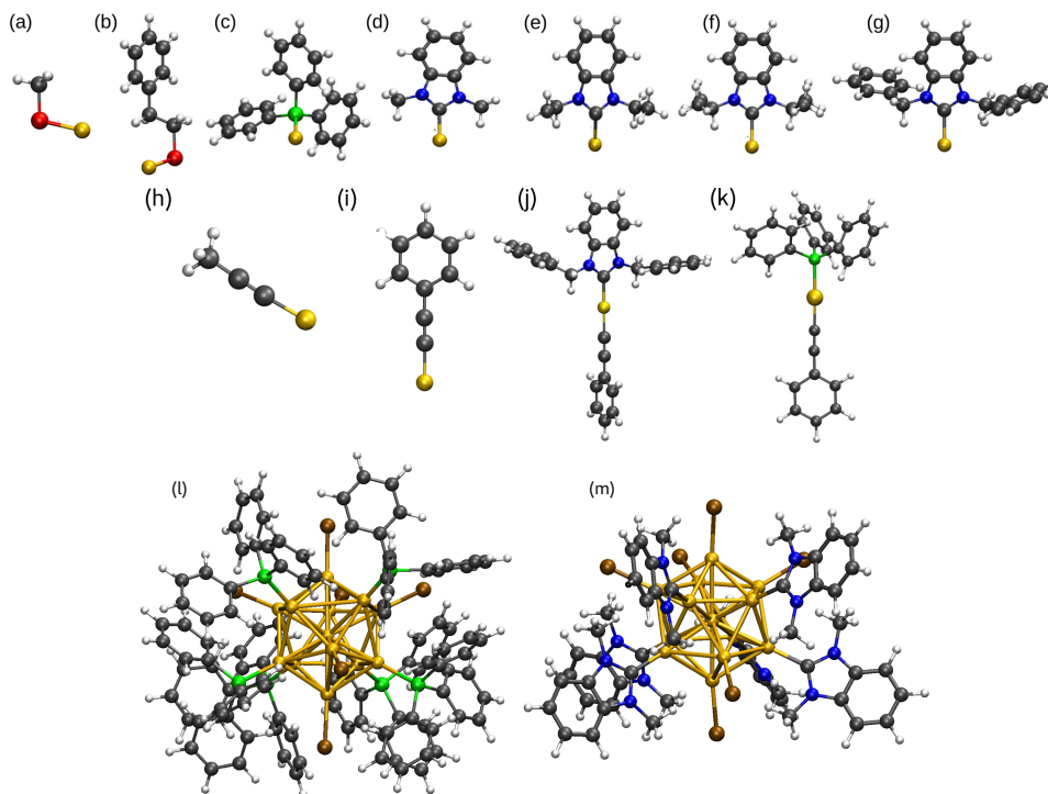
Fig. 1 Molecular structures of PBE optimized M-L complexes (a-i), L 1 -M-L 2 (j and k), and two PPh 3 and NHC Me protected leted metal clusters (l and m, respectively). (a) Au-SCH 3 , (b) Au-SC 8 H 9 , (c) Au-PPh 3 , (d) Au-NHC Me , (e) Au-NHC Et , (f) Au-NHC iPr , (g) Au-NHC Bn , (h) Au-CCMe, (i) Au-CCPh, (j) NHC Bn -Au-CCPh 3 , (k) PPh 3 -Au-CCPh, (l) [Au 13 (PPh 3 ) 6 Br 6 ] - , (m) [Au 13 (NHC Me ) 6 Br 6 ] - . Au, yellow; S, red; C, black; H, white; P, green; N, blue; Br, brown. The optimized structures of Au-L, L 1 -Au-L 2 , and [Au 13 L 6 Br 6 ] - are representative of all M-L and L 1 -M-L 2 complexes and ligand protected metal clusters; the atom radius is not precise.
