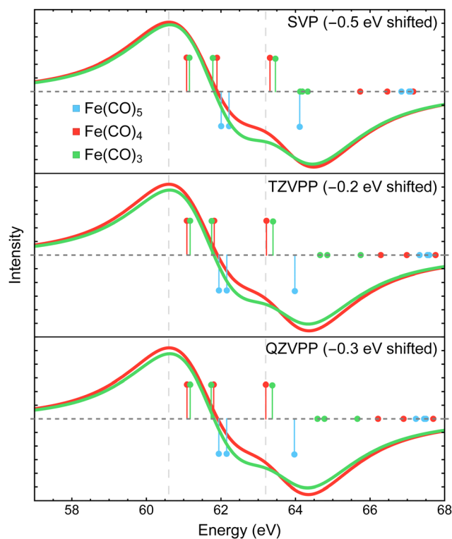
Fig. 10 Difference Fe 3p X-ray photoelectron spectra of \text{Fe}(\text{CO})_4 and \text{Fe}(\text{CO})_3 relative to \text{Fe}(\text{CO})_5 simulated using MR-ADC(2)-X with three fully uncontracted basis sets: def2-SVP, def2-TZVPP, and def2-QZVPP. Vertical lines represent the computed core ionization energies and the corresponding photoelectron intensities. The simulated spectra were shifted to align the position of zero-intensity intercept with the experimental spectrum. Calculations employed the CAS(10e,10o) active space. See Section 3 for more computational details.
