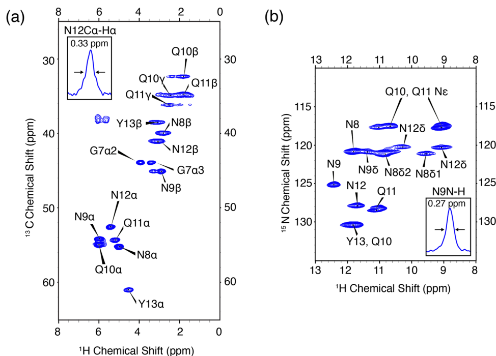
Fig. 2 High resolution ^1\text{H} detected CP-HSQC spectra of nanocrystalline U- ^{13}\text{C} , ^{15}\text{N} -GNNQQNY at \omega_r/2\pi = 90 kHz, \omega_{0\text{H}}/2\pi = 800 MHz. (a) ^1\text{H} - ^{13}\text{C} correlations. (b) ^1\text{H} - ^{15}\text{N} correlations. The mixing times and other spectral acquisition parameters are provided in Table S2 (ESI†).
