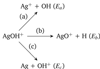
Scheme 1 Dissociation channels of \text{AgOH}^+ cluster.
