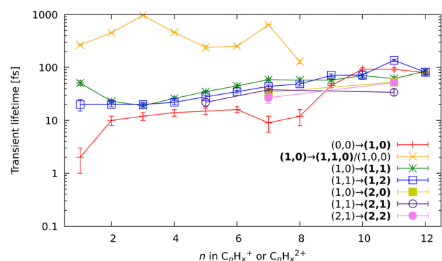
Fig. 9 All fitted relaxation lifetimes of the different fragmentation-related processes, extracted through the global fitting of the pump-probe dependent observables. The x-axis indicates the size of the fragment in which the corresponding lifetime was observed, and the y-axis shows lifetimes on a logarithmic scale. The bold font in the legend indicates in which channel of the fragment ion the transient was observed. The (1, \dots) and (2, \dots) bold channels' notation indicates that the lifetime was observed either in the monocationic or dicationic fragment, respectively.
