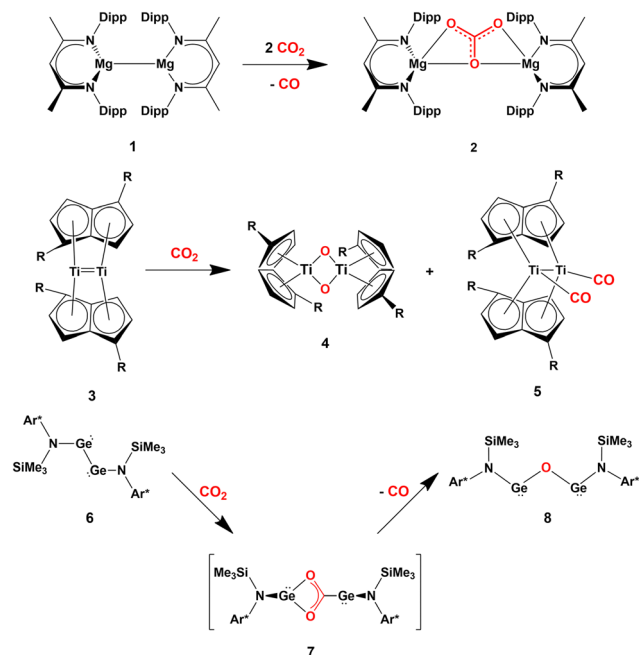
Scheme 1 Relevant examples of cooperative CO 2 activation with s- ( 1 ), d- ( 3 ) and p-block ( 6 ) homobinuclear compounds featuring apolar E–E bonds. (R = Si i Pr 3 ; Ar* = C 6 H 2 (C(H)Ph 2 ) 2 Me-2,6,4).
