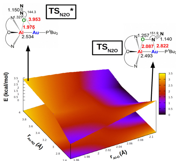
Fig. 6 Potential energy surface (PES) in the region neighbouring the transition state TS for the reaction of complex [\text{tBu}_3\text{PAuAl(NON)}] with \text{N}_2\text{O} . Insets: Position on the PES and schematic structure of TS and \text{TS}^* . Energy has been shifted in each case according to the minimum energy structure. Reproduced with permission from ref. 63 Copyright 2023, Wiley-VCH GmbH.
