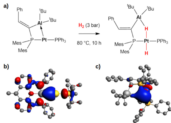
Fig. 5 (a) Experimentally reported reactivity of a Pt \rightarrow Al complex with \text{H}_2 . 52 (b) and (c) Isosurfaces of the HOMO of the gold-aluminy complex (b) and platinum-aluminum complex (c). The isovalue is 3 m_e a_0^{-3} . The isosurfaces have been taken and adapted with permission from ref. 50 Copyright 2023, Royal Society of Chemistry.
