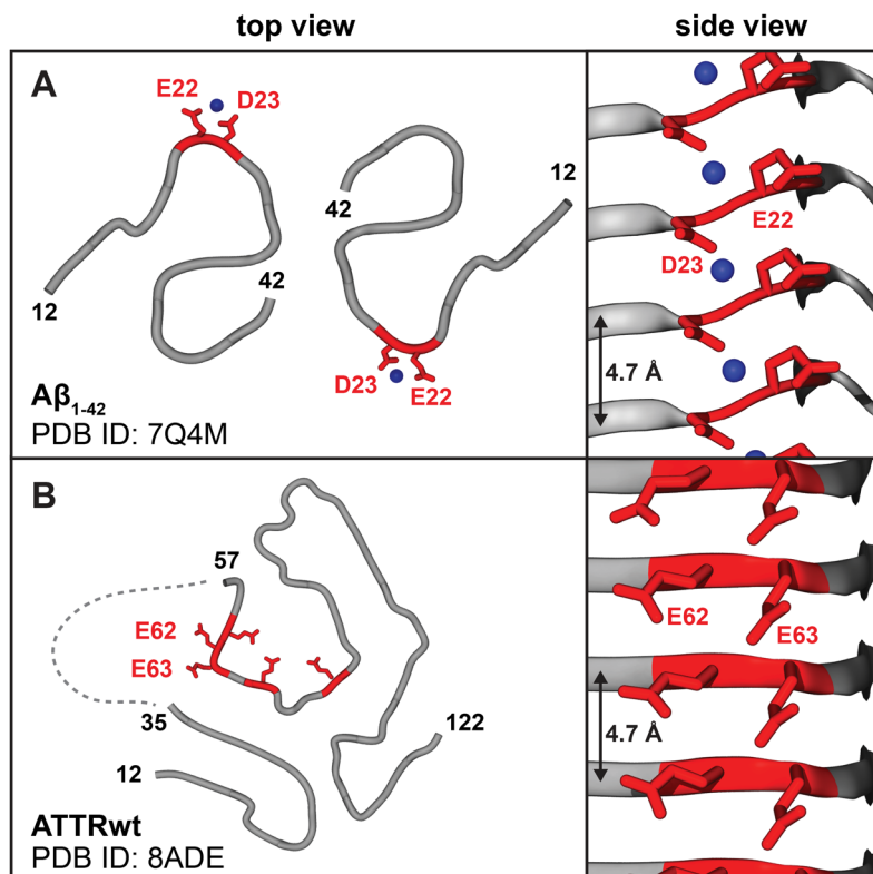
Fig. 2 Amyloids display periodic ligand binding sites on the fibril surface, including acidic residue pairs that can bind calcium. (A) Cryo-EM structures of patient-derived Aβ 1-42 type-I and type-II fibers show periodic arrays of metal ions bound by acidic residue pairs, Glu22-Asp23; 20 type-II fibril structure is shown. (B) Cryo-EM structures of ATTR type-A fibrils feature surface arrays of acidic pairs, e.g. Glu62-Glu63 in the major “closed-gate” polymorph. Linker residues 35–56 are cleaved or disordered (dashed line), 29 providing access to the Glu62-Glu63 site that probably binds Ca 2+ .
