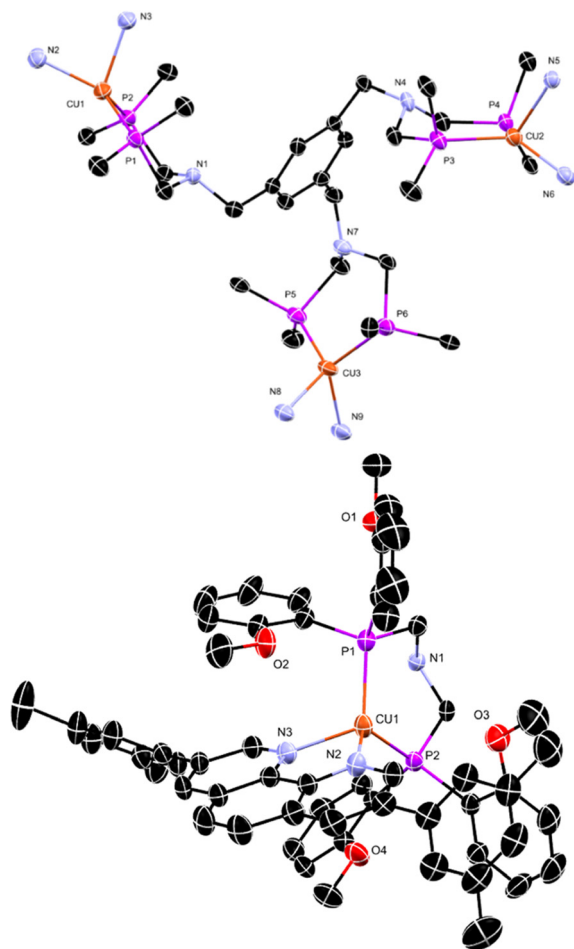
Fig. 1 Crystal structure of [(\text{Cu}(3,8\text{-bis}(3,5\text{-bis(trifluoromethyl)phenyl)}-1,10\text{-phenanthroline)}_3(1,3,5\text{-tris(PNP-methylene)benzene}))(\text{BF}_4)_3] , 4d . Anions, solvent molecules, and protons are omitted for clarity. Above: only the pivot atoms of the anisyl groups and the 3,5-bis(trifluoromethyl)phenyl-1,10-phenanthroline ligands are shown. Below: the steric crowding around the Cu1 centre is shown. The Cu1...O2, Cu1...O3, and Cu1...O4 contact distances are 3.391, 3.423, and 3.358 Å, respectively. O1 is orientated away from the Cu1 centre. Only the carbon pivot atoms of the CF 3 groups are depicted.
