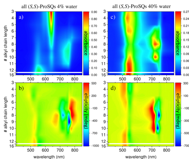
Fig. 2 UV/Vis absorbance spectra (top row) and corresponding ellipticity spectra (bottom row) in a 2D representation of all (S,S)-ProSQ compounds with varying alkyl chain lengths (C3 to C16) for two selected volume-percentages of water in the methanol–water: 4% in (a) and (b) and 40% in (c) and (d).
