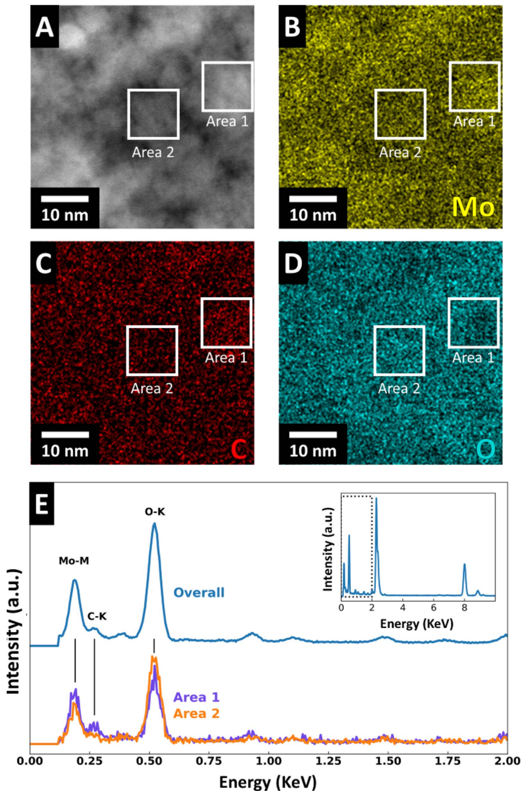
Fig. 5 (A) HAADF-STEM micrograph showing Z-number contrast and (B–D) EDS mapping with elemental distribution of Mo, C, and O in \text{MoO}_x\text{-C} . (E) Chemical analysis of the two marked areas by quantitative STEM-EDS spectral imaging analysis.
