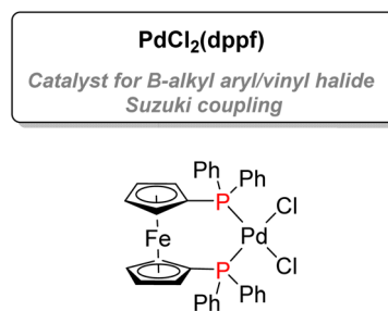
dppf = 1,1'-Bis(diphenylphosphino)ferrocene
