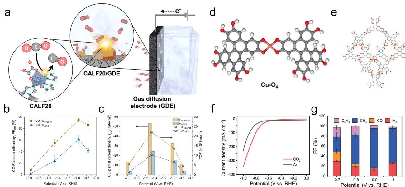
Fig. 6 Zn-based CALF20 features ligand-based active sites (a) whose electron-rich structure facilitates \text{CO}_2\text{R} to CO more than a ZIF-8 analogue (b and c). 87 \text{Cu-O}_4 active sites (d) within a Cu-BTC MOF (e) exhibit both high activity (f) and selectivity (g) for \text{CO}_2\text{R} to \text{CH}_4 . 95 Reproduced with permission from the American Chemical Society, copyright 2021 and Springer Nature, copyright 2021.
