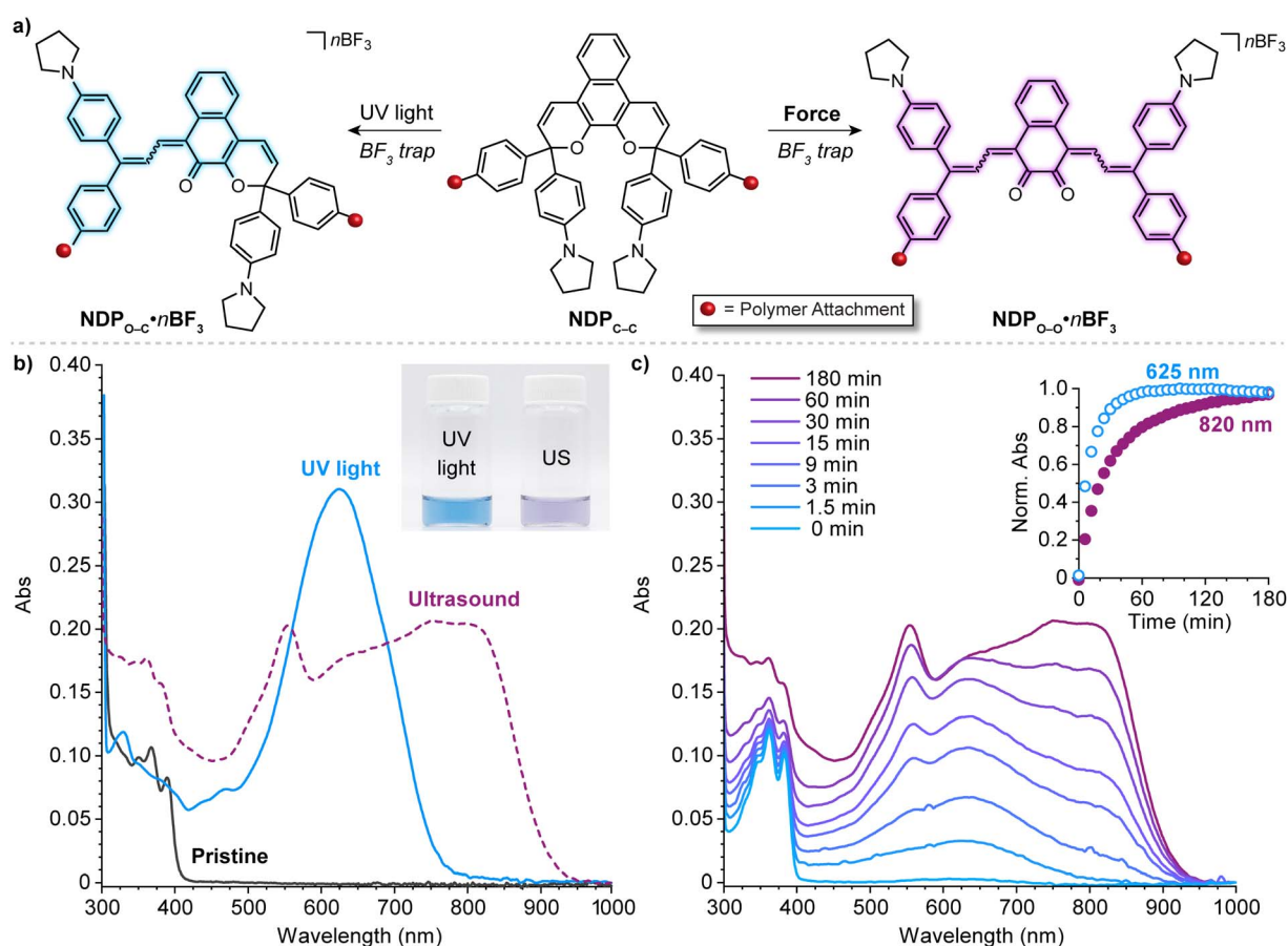
Fig. 13 (a) Divergent photochemical and mechanochemical reactivity of a 3H-naphthodipyran (NDP) moiety incorporated near the center of a poly(methyl acrylate) chain. (b) UV-vis-near-infrared absorption spectra before and after photoirradiation of the polymer with UV light or ultrasound-induced mechanochemical activation. Inset shows a photograph of the two solutions after activation. (c) Absorption spectra recorded during ultrasonication of the polymer and time-dependent absorption profiles at 625 and 820 nm characteristic of monomerocyanine NDP O-C · nBF 3 and dimerocyanine NDP O-O · nBF 3 , respectively. Adapted with permission from ref. 146. Copyright 2022, American Chemical Society.
