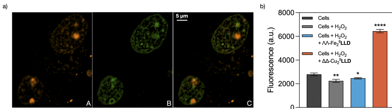
Fig. 6 (a) \Delta\Delta -Cu II TAMRA-LLD selectively stains DNA replication sites at the cell nuclei. Vero cells expressing protein GFP-PCNAL2 were incubated in the presence of 25 \mu\text{g mL}^{-1} of digitonin for 3 min and then in the presence of 5 \mu\text{M} of \Delta\Delta -Cu II TAMRA-LLD for 15 min. The Cu II peptide helicate used in these studies was previously assembled before the internalization experiment by adding 5 eq. of CuCl 2 ·2H 2 O to an aqueous solution of TAMRA-LLD peptide ligand. (A) Red channel emission showing the distribution of the TAMRA-labelled helicate; (B) green channel, corresponding to the emission of the GFP-PCNAL2 probe that labels DNA replication foci; (C) overlay of the green and red channels, which shows that \Delta\Delta -Cu II TAMRA-LLD has localised at the replication foci. Nucleoli are clearly labelled as red spots inside the cell nuclei. The images show a representative confocal section of the Vero cells. (b) Detection of free DNA ends by TUNEL assay. S-phase synchronized Vero cells were incubated with H 2 O 2 alone and with \Lambda\Lambda -Fe II LLD or \Delta\Delta -Cu II LLD plus H 2 O 2 at 37 °C for 2 hours and then subjected to TUNEL analysis for the detection of free DNA ends. Results are represented as the mean with standard deviation of a triplicate experiment * = P \leq 0.05 ** = P \leq 0.01 *** = P \leq 0.001 and **** = P \leq 0.0001 .
