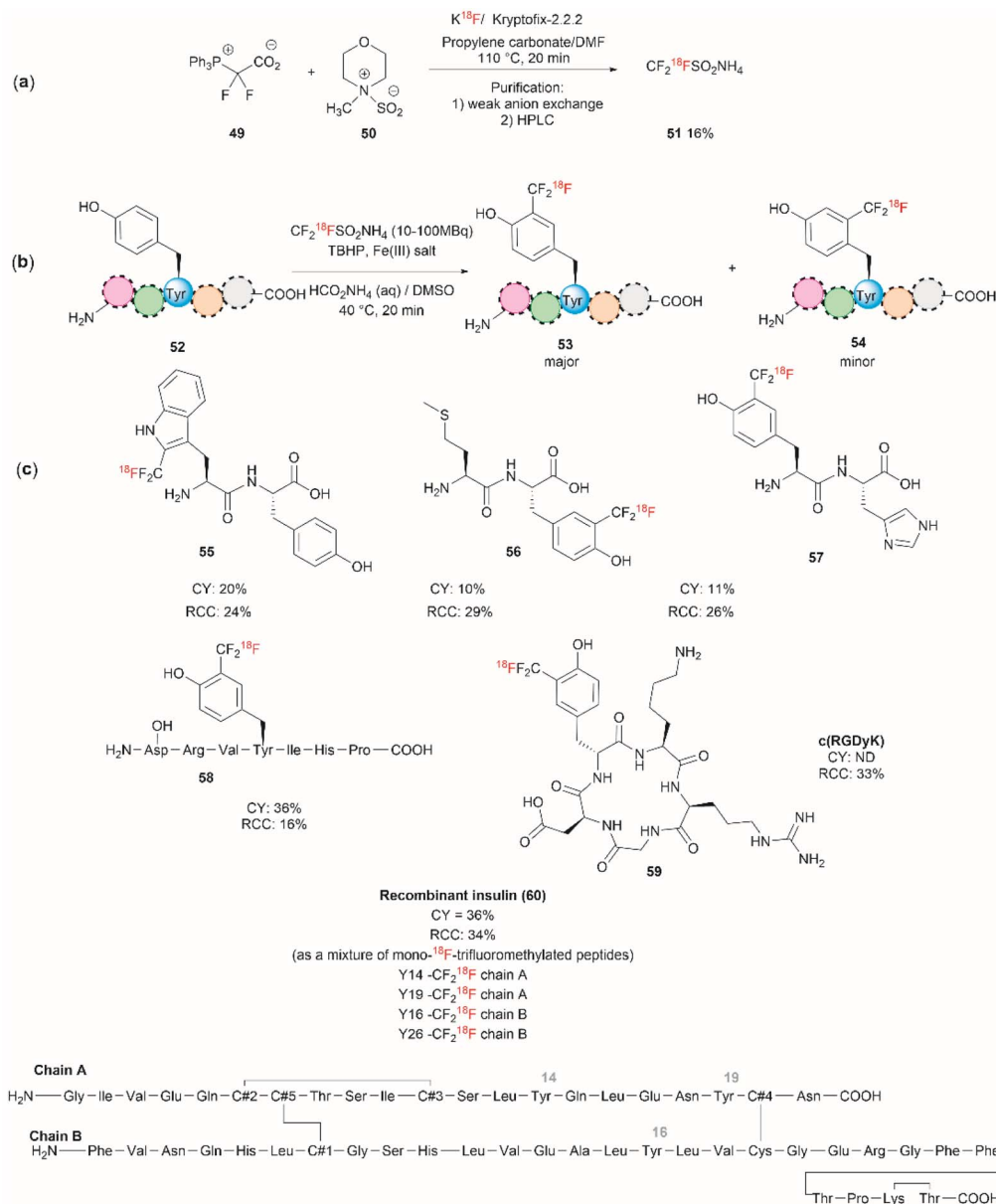
Fig. 13 (a) Chemical synthesis of ammonium 18 F-trifluoromethanesulfonate. (b) General conditions for the 18 F-trifluoromethylation of Tyr containing peptides. (c) 18 F-trifluoromethylated peptides.
