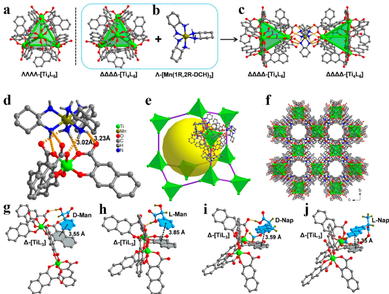
Fig. 23 (a) Molecular structures of the \Delta\Delta\Delta\Delta -[Ti 4 L 6 ] and \Lambda\Lambda\Lambda\Lambda -[Ti 4 L 6 ] enantiomers. (b) \Lambda -[Mn(1 R ,2 R -DCH) 3 ] unit in PTC-108(Δ). (c) Two adjacent \Delta\Delta\Delta\Delta -[Ti 4 L 6 ] cages linked by one \Lambda -[Mn(1 R ,2 R -DCH) 3 ] unit. (d) N-H...O H-bonds in PTC-108(Δ). (e and f) Diamondoid cage and 3D framework of PTC-108(Δ). (Ti, green; Mn, olive; O, red; N, blue; C, gray). (g–j) Illustration of the proposed recognition models of the PTC-108(Δ) cage towards enantiomers. 70 Reproduced with permission from ref. 70. Copyright 2018, the American Chemical Society.
