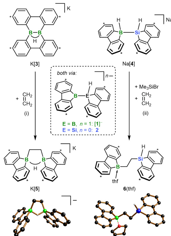
Scheme 2 Diboration and silaboration of ethylene, starting from K[3] or Na[4]/Me_3SiBr and furnishing K[5] and 6 (thf), respectively. The reactions proceed via the valence isoelectronic intermediates [1]^- and 2 . (i) THF- d_8 , -196 \text{ }^\circ\text{C} to RT, 99% yield; (ii) THF, -78 \text{ }^\circ\text{C} to RT, 56% yield. Carbon atoms marked with "*" bear t Bu groups. In the crystal-structure plots, the [K(thf)_2]^+ counter cation of [5]^- , C-bonded H atoms, and Ar-bonded t Bu groups are omitted for clarity; H: gray, B: green, C: black, O: red, Si: blue.
