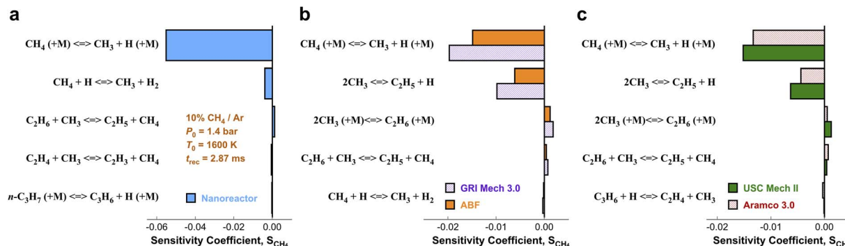
Fig. 4 Ranked sensitivity bar chart for CH_4 mole fraction with respect to reaction rates computed under condition 10% CH_4/Ar , P_0 = 1.4 bar, T_0 = 1600 K, and t_{rec} = 2.87 ms. Five reaction kinetic models are analyzed, including (a) the nanoreactor, (b) GRI Mech 3.0 & ABF, (c) USC Mech II & Aramco 3.0.
