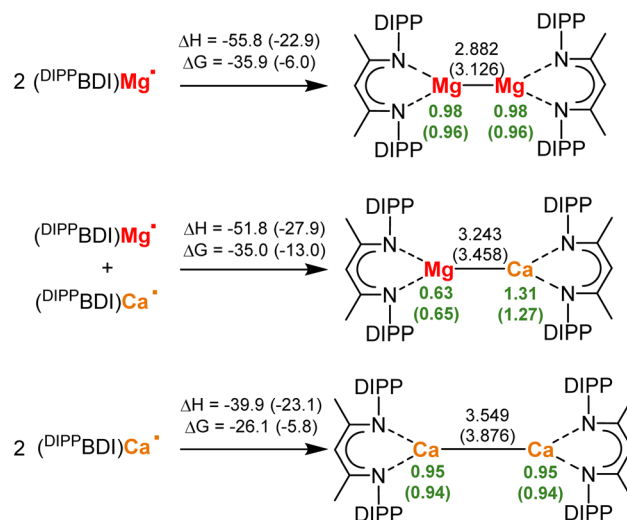
Scheme 2 Formation of homo- and hetero-metallic (^{\text{DIPP}}\text{BDI})\text{Ae}^{\text{II}}\text{Ae}^{\text{II}}(^{\text{DIPP}}\text{BDI}) complexes (Ae = Mg or Ca). Enthalpies and Gibbs free energies at 298 K in \text{kcal mol}^{-1} , Ae–Ae distances in Å and NPA charges in green; B3PW91/def2TZVP//def2SVP with dispersion correction (GD3BJ). Values in brackets relate to calculations without dispersion corrections.
