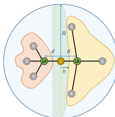
Fig. 7 Illustration of eqn (1) with % V_{\text{Bur\_LA}} , % V_{\text{Bur\_LB}} , and % V_{\text{corr}} .
