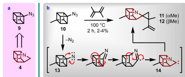
Scheme 1 (a) Retrosynthesis of 4 from 9. (b) Synthesis of spirocyclopropyl methyl azahomocubane (11 and 12; diastereomers tentatively assigned) via nitrene 14.
