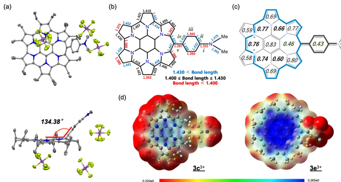
Fig. 7 (a) Crystal structures (top and side views) of 3\mathbf{c}^{3+}[\text{SbF}_6^-]_3 . Thermal ellipsoids are scaled to 50% probability. Solvent molecules and disordered atoms are omitted for clarity. (b) Selected bond lengths (Å) and (c) HOMA values of the crystal structure of 3\mathbf{c}^{3+}[\text{SbF}_6^-]_3 . (d) ESP plots of 3\mathbf{c}^{3+} and 3\mathbf{e}^{3+} calculated at the B3LYP/6-31G(d) level of theory, in which the Et groups are replaced with Me groups to simplify the calculations.
