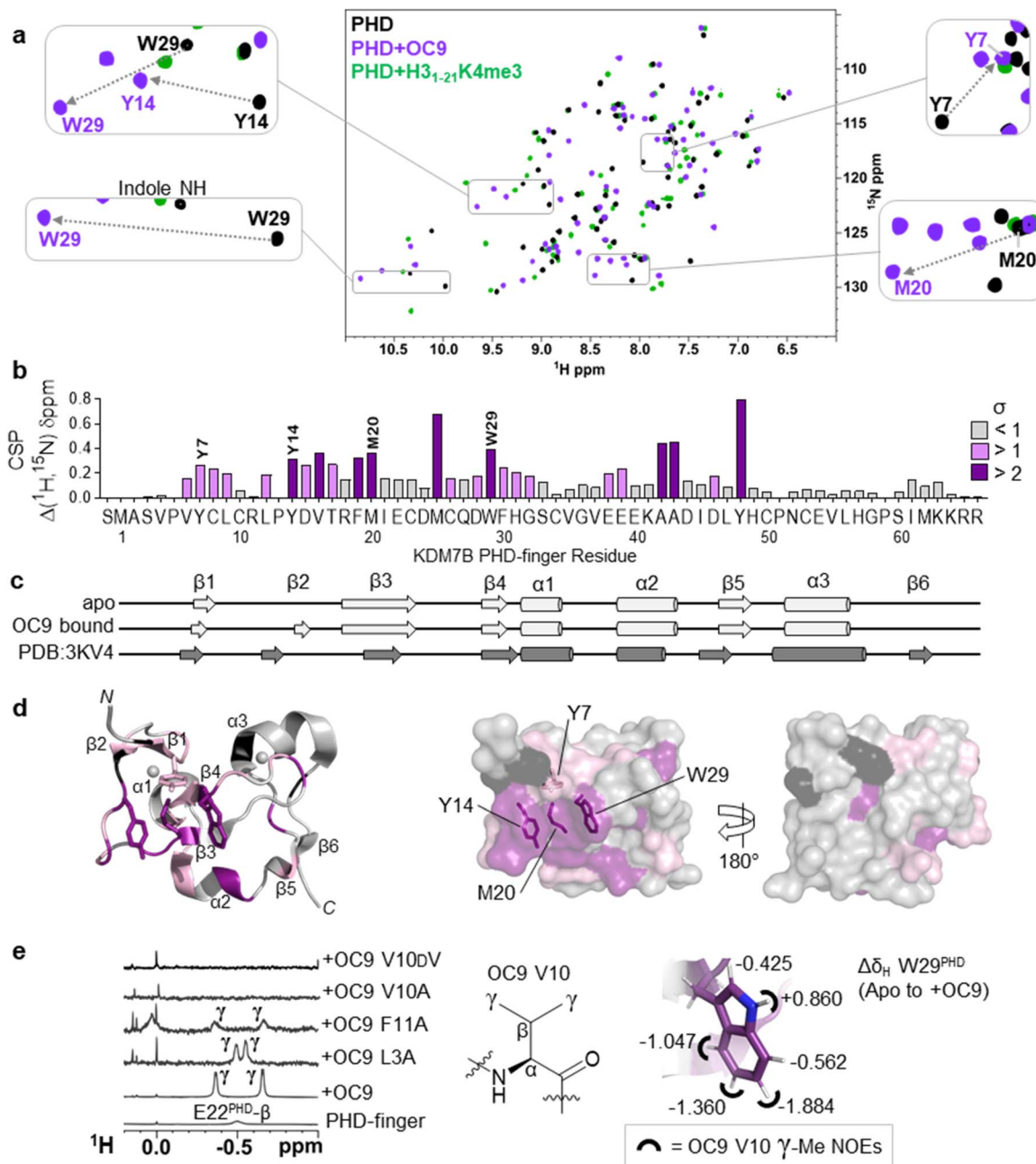
Fig. 4 Protein NMR reveals valine contacting of the aromatic cage. (a) ^1\text{H} - ^{15}\text{N} HSQC of KDM7B PHD-finger in the apo (black) or bound forms with OC9 (purple, 1 : 1) or H 3_{1-21} K4me3 (green, 3 : 1). (b) ^1\text{H} and ^{15}\text{N} chemical shift changes for apo vs. + OC9 were combined and weighted to give chemical shift perturbation (CSP) ( \Delta\delta ) values. Standard deviation ( \sigma ) of \Delta\delta are indicated (>1 pink, >2 purple). (c) TALOS+ predicts similar secondary structure elements in apo and OC9-bound solution protein complexes (light grey) to those found in PDB ID 3KV4 (dark grey). (d) Mapping of CSP \sigma from (b) onto PDB ID 3KV4 shows OC9 binding surfaces primarily along one face, which presents the cage (annotated residues). (e) Shielded ^1\text{H} -NMR signals centred around -0.5 ppm belonging to the OC9 V10 \gamma -methyl groups are observed in some OC9-PHD complexes, but not in apo protein, or complexes with OC9 V10A and OC9 V10 \Delta V. The V10 OC9 \gamma -methyl signals have NOE interactions (black semi-circles) with the W29 PHD indole, which itself is shielded upon binding of OC9 (indicated by \Delta\delta_{\text{H}} values).
