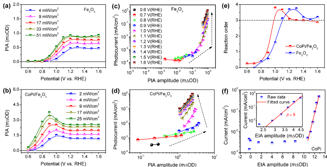
Fig. 5 Light-intensity-dependent PIA spectra of (a) bare Fe 2 O 3 and (b) CoPi/Fe 2 O 3 at increased potential. Pump wavelength is 456 nm; probe wavelength is 694.3 nm. Rate law analysis for (c) Fe 2 O 3 and (d) CoPi/Fe 2 O 3 . The colors of lines at various potentials in (c and d) are identical. (e) Reaction order of the two photoanodes as a function of potential. (f) Log(current) versus hole density from EIA spectra for the CoPi electrocatalyst. The inset shows the rate law analysis with corrected hole density for the CoPi electrocatalyst.
