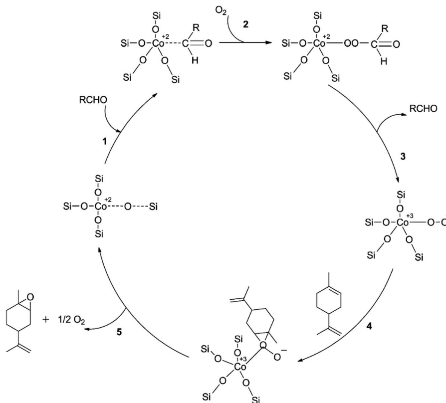
Scheme 9 A proposed method for limonene aerobic oxidation reproduced from ref. 50.
