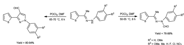
Scheme 6 Synthesis of ( E )- N -(aryl)- N -(1-thiophen-2-yl)ethylidene formylhydrazone and 3-(thiophen-2-yl)-1 H -pyrazole-4-carbaldehydes.
