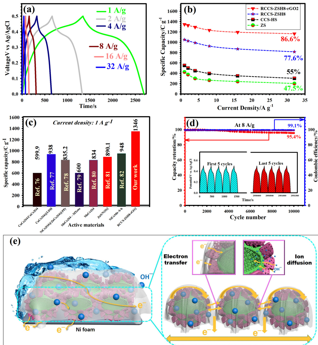
Fig. 7 (a) GCD profiles of the RCCS-ZSH8-rGO2 electrode from 1 to 32\ A\ g^{-1} . (b) Specific capacities vs. current densities of the ZS, CCS-HS, RCCS-ZSH8, and RCCS-ZSH8-rGO2 electrodes. (c) Comparison of capacity values of RCCS-ZSH8-rGO2 with the previous literature. (d) Longevity and Coulombic efficiency of the RCCS-ZSH8-rGO2 at 8\ A\ g^{-1} (the inset depicts the first and last 5 GCD cycles). (e) Schematic representation of the working mechanism of RCCS-ZSH8-rGO2 base-electrode.
