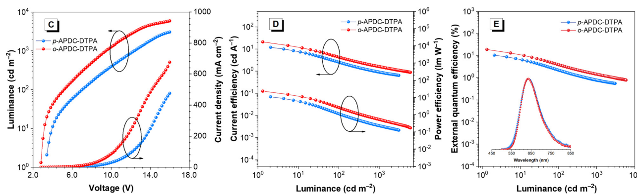
Fig. 4 (A) Device structures and energy level diagrams of non-doped and doped devices. (B) Molecular structures of the materials employed in the devices. (C) Luminance–voltage–current density, (D) current efficiency–luminance–power efficiency and (E) external quantum efficiency–luminance of the doped OLEDs with a concentration of 10 wt% in the TPBi host. Inset in plane E: EL spectra of the doped OLEDs.
