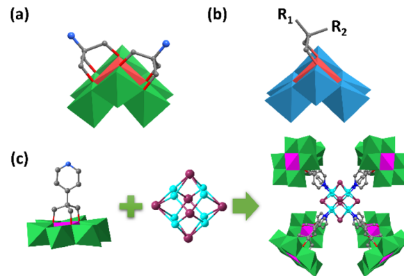
Fig. 5 (a) Schematic diagram of the \{[H_3NC(CH_2O)_3]_2MnMo_6O_{18}\}^- structure. (b) Schematic diagram of the \{[R_1R_2C(CH_2O)_2]Mn^IVW_6O_{22}\}^{6-} structure. (c) Synthesis diagram of [TBA]_{14}[Cu_8I_6][HCr(OH)_3Mo_6O_{18}L_3]_8 . Color code: {MoO 6 }, green octahedron; {MnO 6 }, red octahedron; {WO 6 }, blue octahedron; {CrO 6 }, pink octahedron; C, gray; N, light blue; Cu, turquoise; I, purple.
