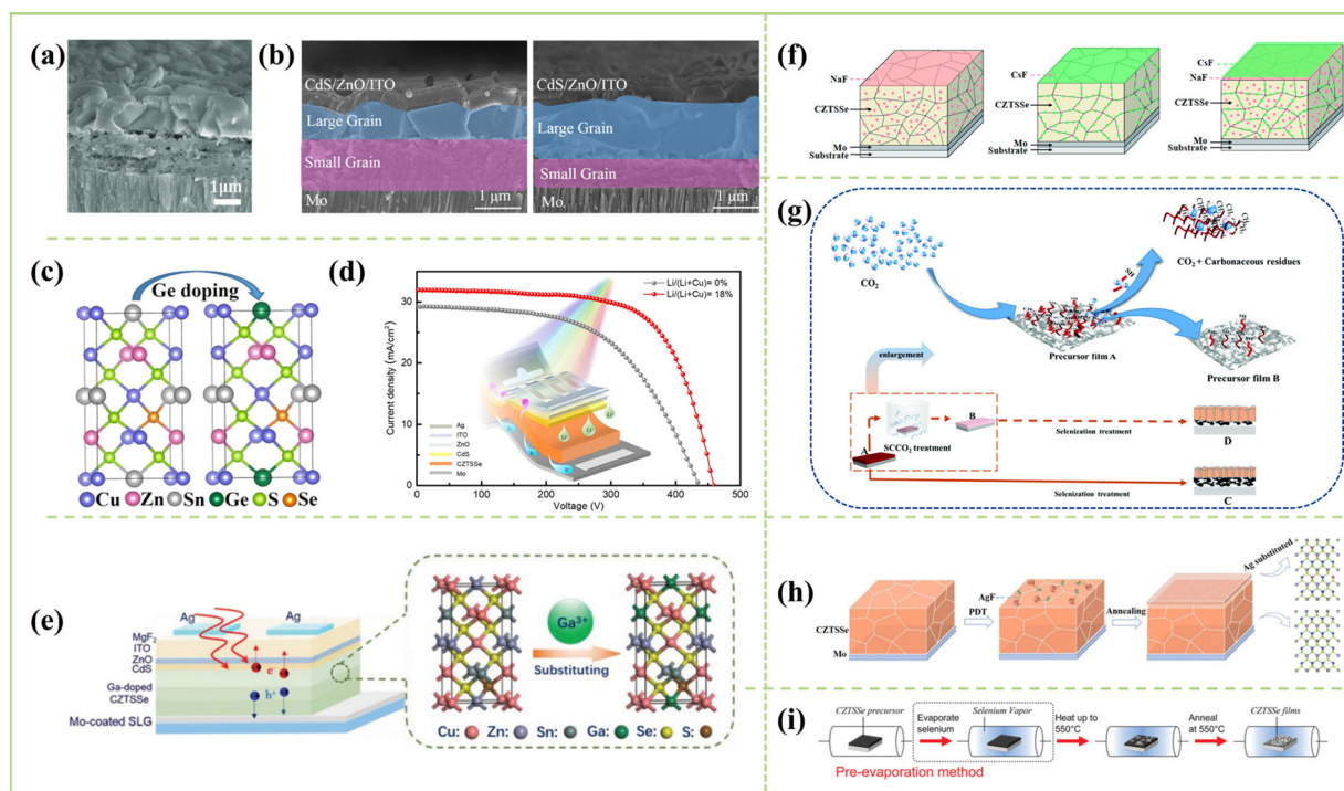
Fig. 5 (a) The cross-section SEM image of flexible \text{Cu}_2\text{Zn}_{1-x}\text{CdSn}(\text{S,Se})_4 solar cells. 75 Copyright © 2019, WILEY-VCH Verlag GmbH & Co. KGaA. (b) The cross-sectional SEM images of reference (left) and 15 nm Ge samples (right). 76 Copyright © 2021, Elsevier. (c) Schematic of CZTGSSe solar cell with the model of doping \text{Ge}^{4+} : replacing \text{Sn}^{4+} . 76 Copyright © 2021, Elsevier. (d) Main structure diagram of the flexible CZTSe solar cell and J–V curves. 77 Copyright © 2022, Elsevier. (e) Schematic structure of CZTGSSe solar cell and the model of doping \text{Ga}^{3+} : replacing \text{Zn}^{2+} and \text{Sn}^{4+} . 78 Copyright © 2021, Wiley-VCH GmbH. (f) Left–right: schematic diagrams of the alkali element distribution within the Na, Cs, and Na–Cs incorporated CZTSe absorber; the pink and green dots represent Na and Cs atoms, respectively. 79 Copyright © 2021, Royal Society of Chemistry. (g) Schematic illustration of \text{SCCO}_2 treatment on CZTSe film fabrication. 80 Copyright © 2020, Royal Society of Chemistry. (h) Schematic of typical operation procedures for the preparation of AgF-PDT CZTSe absorber. 81 Copyright © 2022, Elsevier. (i) Schematic diagram of pre-evaporation selenization (PES) method. 82 Copyright © 2022, Wiley-VCH GmbH.
