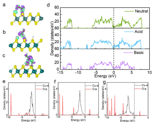
Fig. 4 Charge density difference for \text{H}_2\text{O}_2 adsorption on \text{Cu@MoS}_2\text{-Vs} in (a) neutral, (b) acidic and (c) basic conditions, respectively. The isosurface value of electron density was taken as 0.002 \text{ e } \text{\AA}^{-3} . The cyan and purple regions for the charge density difference represent the areas of electron accumulation and depletion, respectively. (d) TDOS of \text{Cu@MoS}_2\text{-Vs} in different conditions of acidity and alkalinity. (e and f) PDOS of Cu-d and O-p orbitals of \text{Cu@MoS}_2\text{-Vs} in (e) neutral, (f) acidic and (g) alkaline conditions.
