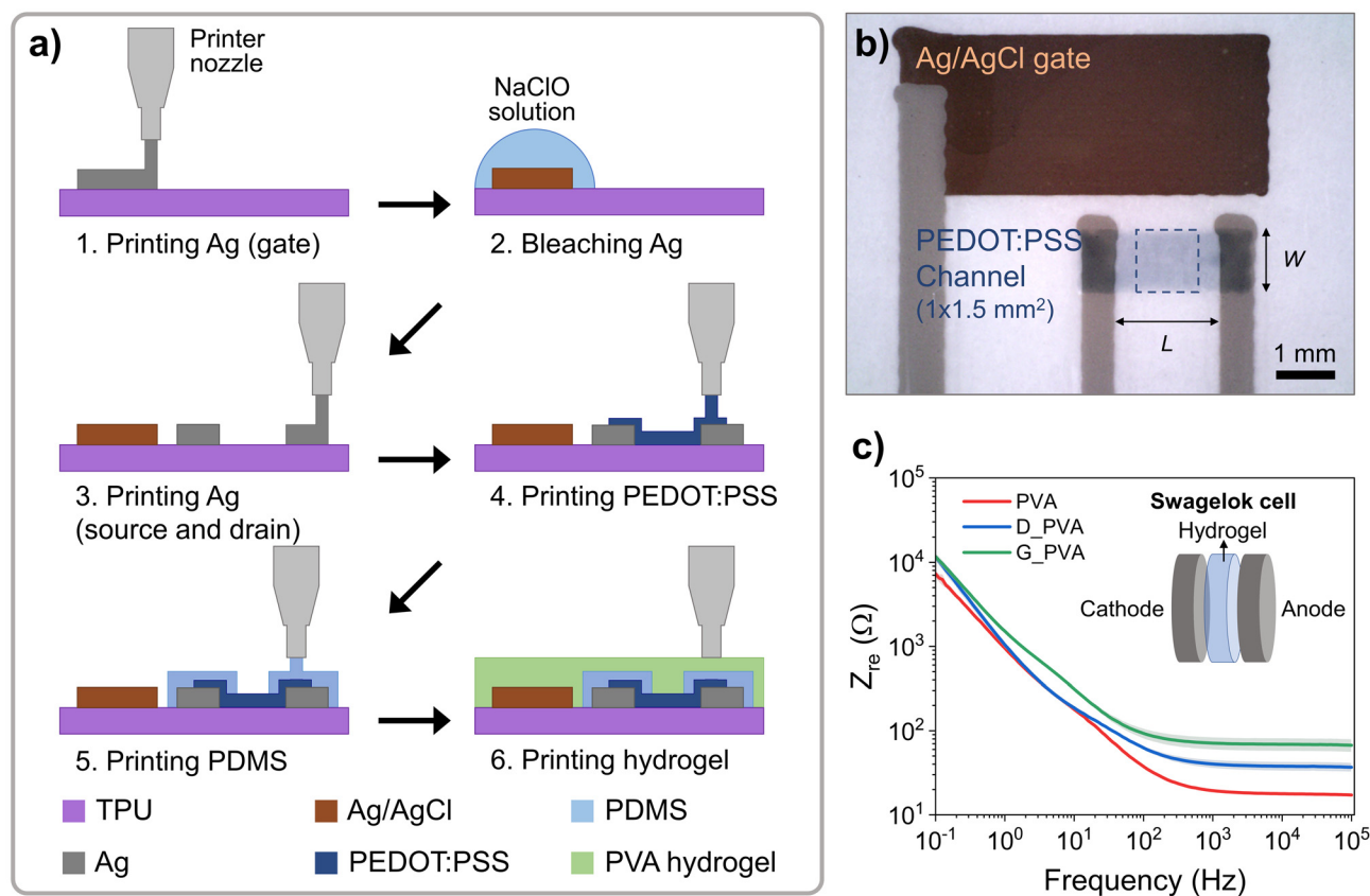
Fig. 1 (a) Process flow to fabricate the printed OEECTs. Step 1: printing stretchable Ag paste as gate electrode on TPU substrate. Step 2: bleaching the printed Ag with NaClO solution to form Ag/AgCl on the surface (thickness \sim 20 \mu\text{m} including a \sim 5 \mu\text{m} AgCl layer). Step 3: printing the Ag source, drain, and interconnects (thickness \sim 20 \mu\text{m} ). Step 4: printing of the PEDOT:PSS channel (thickness \sim 1 \mu\text{m} ). Step 5: printing PDMS to cover source, drain, gate interconnects and the overlap region of PEDOT:PSS with Ag. Step 6: printing hydrogel electrolytes over the gate and channel. (b) Microscopic image of the device. The dashed area indicates the area of the channel ( 1 \times 1 \text{ mm}^2 ), which is not covered by PDMS. (c) Electrochemical impedance ( Z_{\text{re}} ) of the PVA-based hydrogel electrolytes from 10^5 to 10^{-1} Hz, using Swagelok cell. The solid lines are the average values measured from 3 different samples and the shaded area shows the error bars, which represent standard deviation. Since the standard deviation is very small, the shaded area is imperceptible in the graph.
