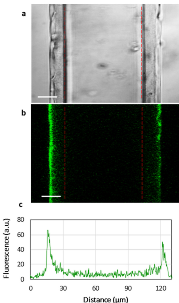
Fig. 4 Light transmittance (a) and confocal (b) images and diametric fluorescence profile (c) of (HA/PLL280) 24 multilayers deposited on fiber glass and incubated with a suspension of PC-PG NBD liposomes (50 \mu\text{M} total lipids in Tris buffer solution at pH 7.4) for 20 minutes. Scale bar is 20 \mu\text{m} . The surface of the glass fibers is marked with red lines.
