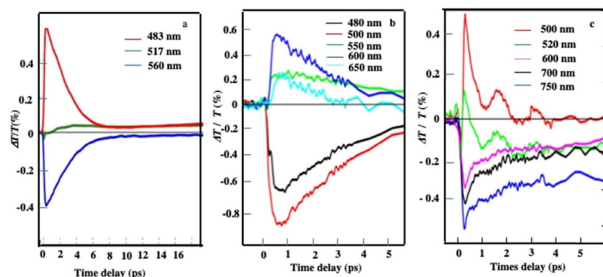
Fig. 10 Dynamics of \Delta T/T at selected probe wavelengths, at short time scales of energy flow in the supraballs, (a) Au "egg" structure (b) and Au/ \text{Fe}_3\text{O}_4 "egg" structures (c). Source: A. Mazanti et al. , 38 PNAS and Schirato et al. , 56 ACS .
