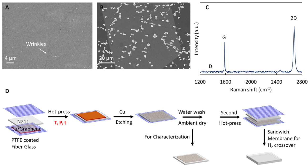
Fig. 1 SEM image of (A) as synthesized graphene on Cu foil, and (B) etch pits on graphene|Cu after 5 s acid etch test with 0.1 M \text{FeCl}_3 . (C) Raman spectrum of graphene transferred onto 300 nm \text{SiO}_2/\text{Si} substrate and (D) schematic of graphene transfer process to Nafion (N211).
