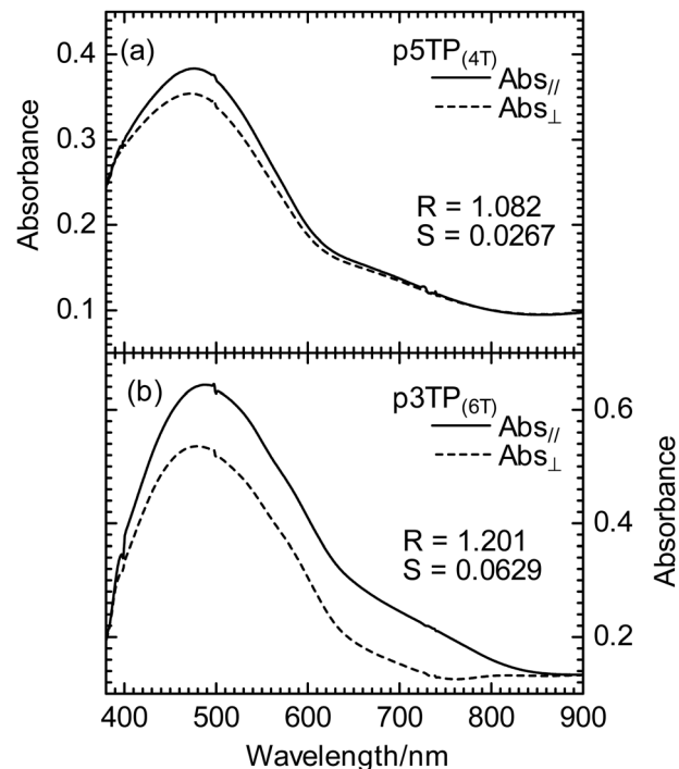
Fig. 3 Linearly polarized UV-vis absorption spectra of (a) p5TP (4T) and (b) p3TP (6T) prepared via electrochemical polymerization in a CLC under a magnetic field. A_{\parallel} , A_{\perp} : absorbance parallel and perpendicular to the magnetic direction, respectively.
