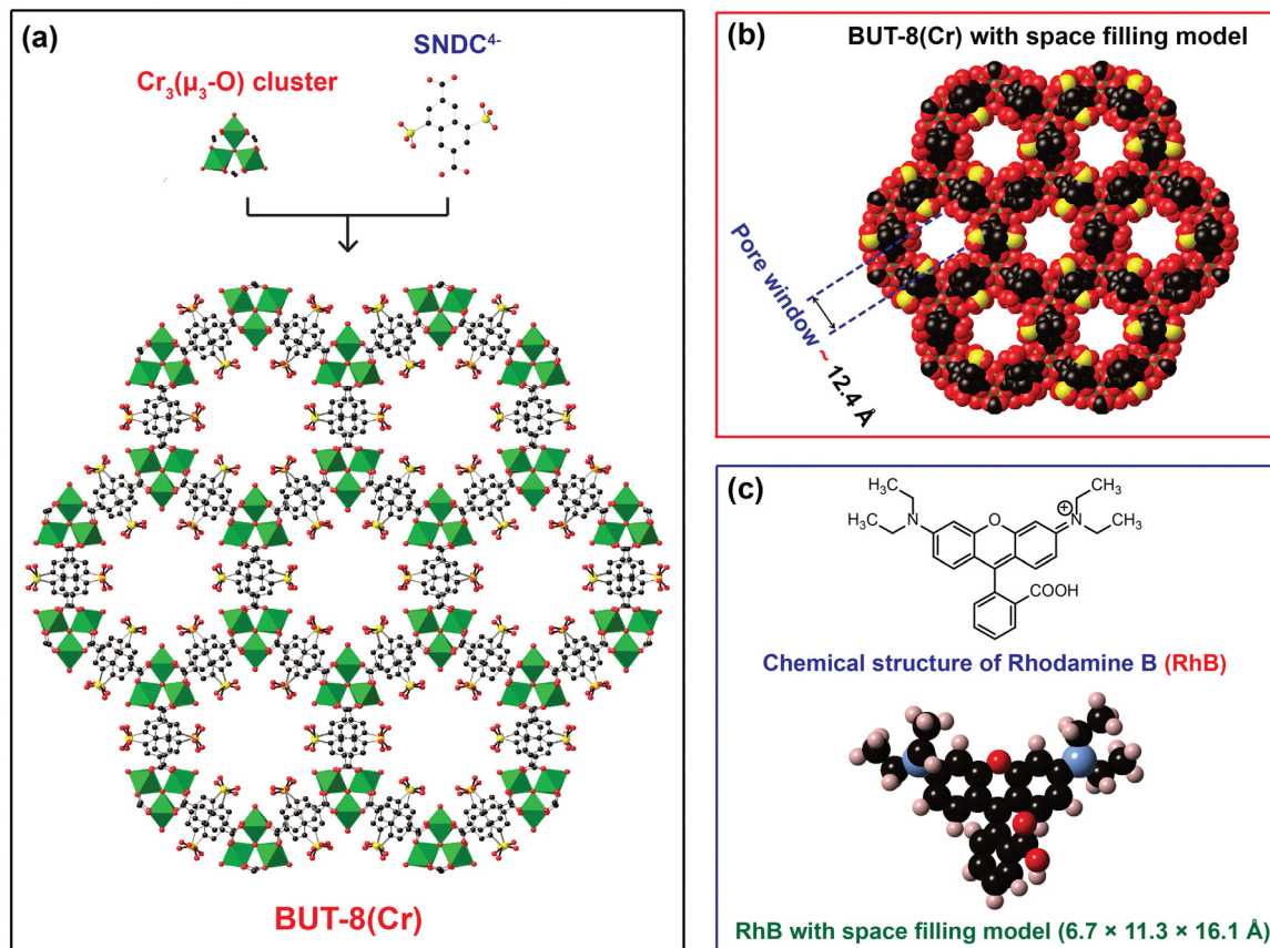
Fig. 1 The structure of \text{H}^+@ BUT-8(Cr) constructed from the \text{Cr}_3(\mu_3\text{-O}) clusters and \text{SNDC}^{4-} linker (a); the pore window of BUT-8(Cr) with the space filling model (b); the chemical structure and space filling model of RhB (c). Atom colors: Cr, green polyhedra; C, black; O, red; S, yellow; N, blue. Almost H atoms are omitted for clarity.
