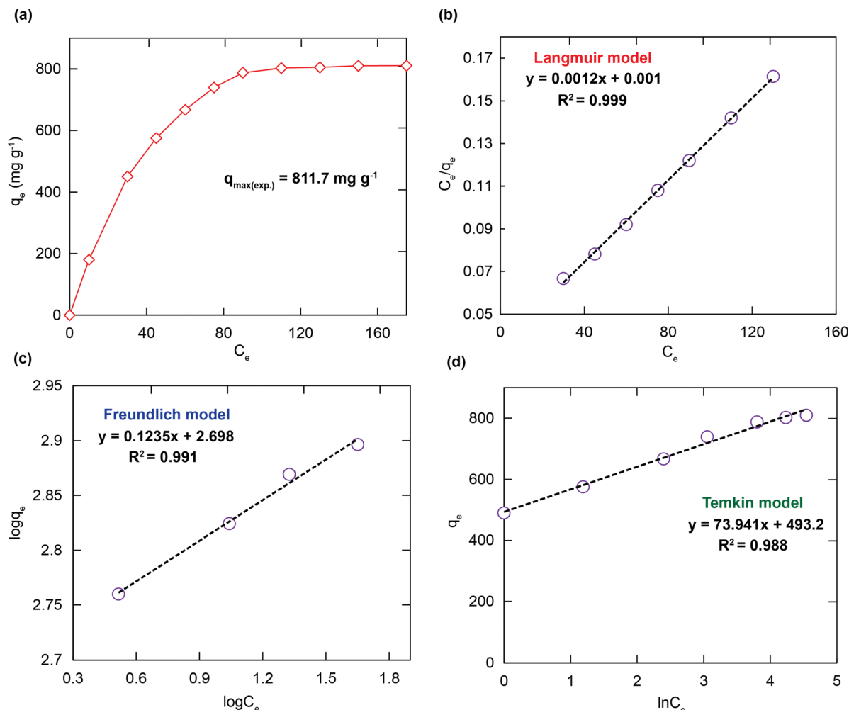
Fig. 5 Effect of the concentration of RhB on the adsorption capacity of H^+cBUT-8(Cr) [ m = 10 mg, V_{RhB} = 100 mL, C_o : 25–175 mg L^{-1} , pH = 3, t = 24 h] (a); fitting results with the adsorption isotherm models: Langmuir (b), Freundlich (c), and Temkin (d).
