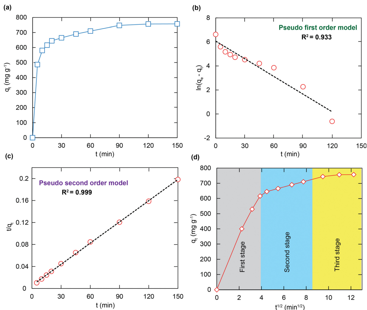
Fig. 6 The kinetic curve for the adsorption of RhB onto \text{H}^+\text{-BUT-8(Cr)} [ m = 10 \text{ mg} , V_{\text{RhB}} = 100 \text{ mL} , C_0 = 100 \text{ mg L}^{-1} , \text{pH} = 3 ] (a); data fitting with the adsorption kinetic models: pseudo first order (b), pseudo second order (c) and intra-particle diffusion model (d).
