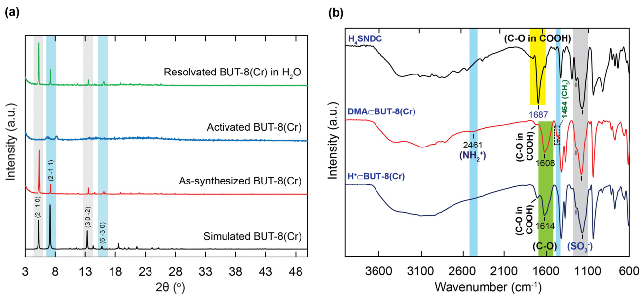
Fig. 2 Powder X-ray diffraction analysis of the as-synthesized DMA@BUT-8(Cr) (red), activated \text{H}^+@ BUT-8(Cr) (blue), and resolved \text{H}^+@ BUT-8(Cr) in water (green) in comparison with simulated BUT-8(Cr) (black) (a); Fourier transform infrared spectra of the \text{H}_4\text{SNDC} linker (black), DMA@BUT-8(Cr) (red), and \text{H}^+@ BUT-8(Cr) (blue) (b).
