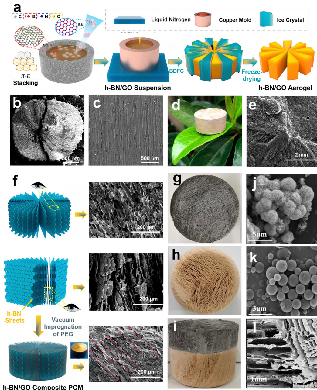
Fig. 8 (a) Schematic illustration of BDFC approach for preparing bioinspired h-BN/GO aerogel. (b) Vertically and (c) radially aligned channels of the water transportation system within towering conifer trees. (d) Optical images of h-BN/GO aerogel. (e) Cross-sectional morphology of the corresponding aerogel. (f) Schematic and SEM images of the cross-sectional and longitudinal section of the h-BN/GO scaffold before and after PCM impregnation. (a–f) Reproduced with permission, 281 Copyright 2020, American Chemical Society. (g–i) Optical images of bilayer aerogel systems. (j–l) SEM images of (j) MoS 2 and (k) paraffin/SiO 2 aerogel-based phase change microcapsules and (l) MMT aerogels. (g–l) Reproduced with permission, 285 Copyright 2022, Elsevier.
