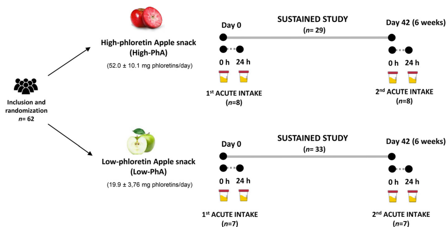
Fig. 1 Study design of acute and sustained interventions with a low-phloretin or a high-phloretin freeze-dried apple snacks.
