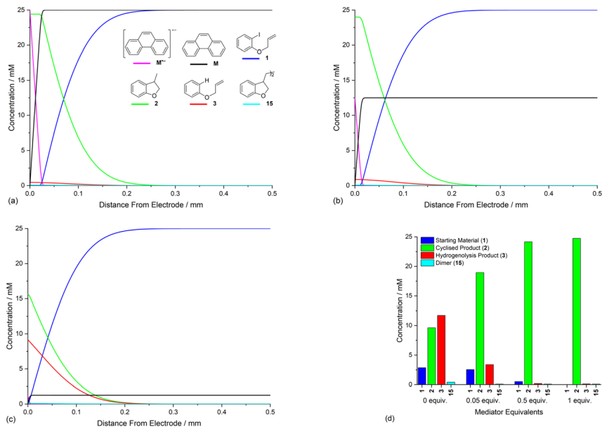
Fig. 6 Influence of mediator (phenanthrene, M) stoichiometry on reaction layer detachment. Concentration profiles for species 1, 2, 3, 15, M and M + for simulated electrolysis under constant potential of -2.8 V vs. SCE at t = 1 s. (a) 1 equiv. of M. (b) 0.5 equiv. of M. (c) 0.05 equiv. of M. (d) Product selectivity profile from simulations with different mediator loadings after electrolysis for 60 s.
